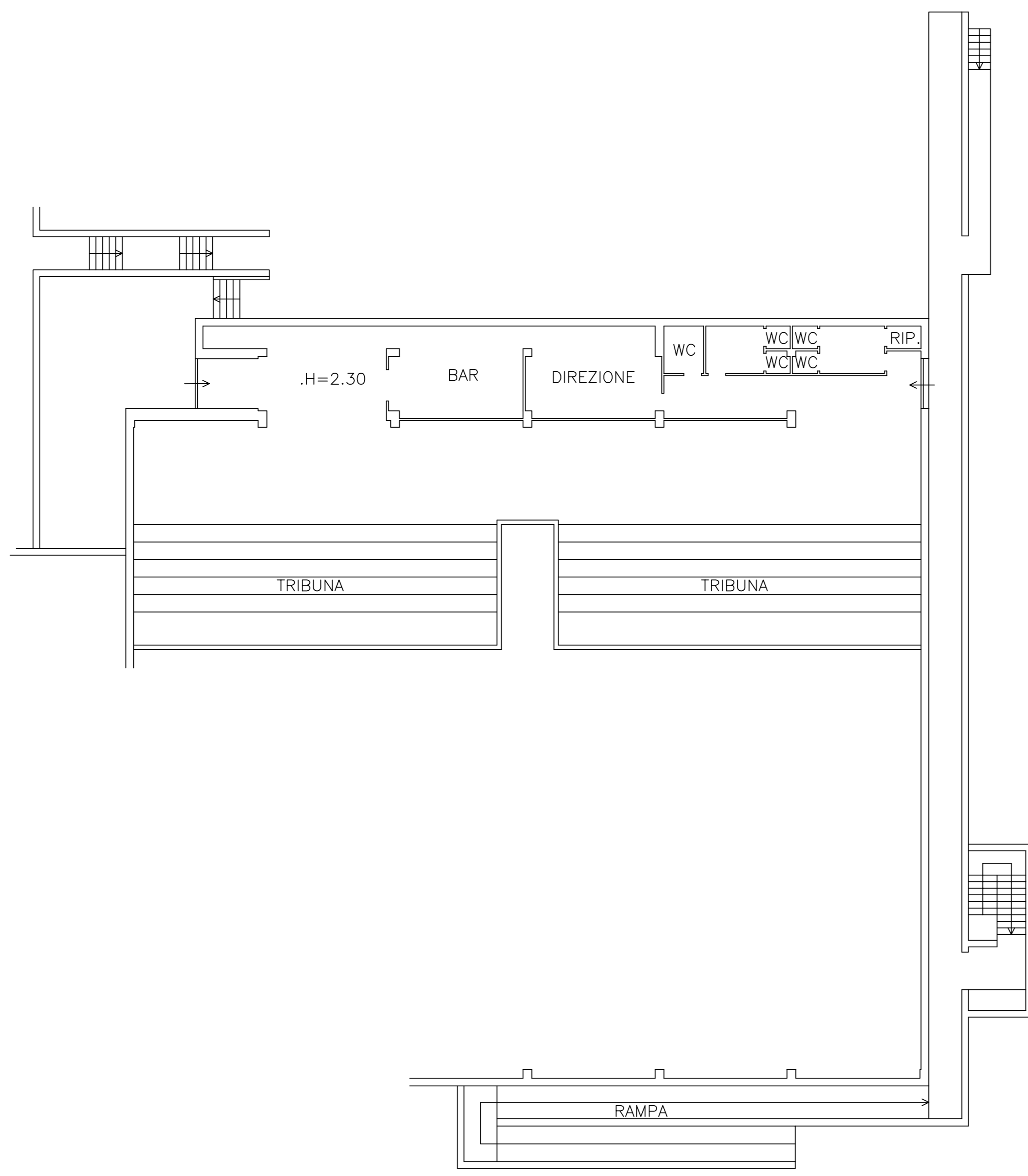
PIANO 1
